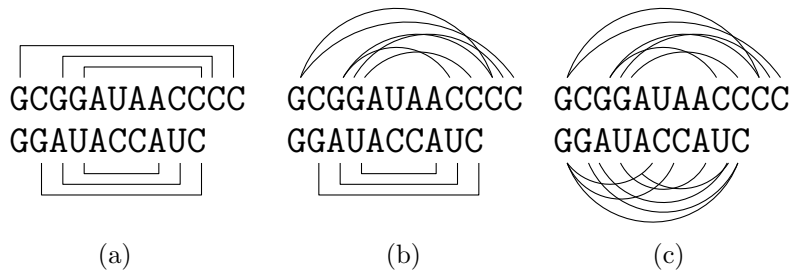
Figure 2: Different input alignment scenarios of RNA sequences (pairwise case): (a) the alignment of two known structures, (b) of one known and one unknown structure, and (c) of two unknown structures.
