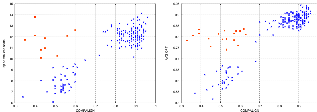
Figure 13: All BRALIBASE k10 instances of low pairwise sequence identity where each cross or box corresponds to one instance: The x-axis gives the Compalign score. The y-axis codes either a structure-normalized score (left side), or the optimality ratio (right side). The red boxes mark the outliers.
