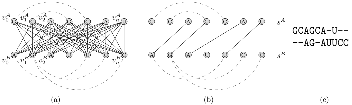
Figure 6: (a) Initial graph model representing two annotated sequences s^A = \text{GCAGCAU} and s^B = \text{AGAUUCC} . Solid lines represent lines, dashed lines represent interaction edges. Please note that in this toy example minimum loop lengths constraints on the interaction edges are violated for sake of compactness of the illustration. Interactions (v_1^B, v_{n-1}^B) and (v_1^B, v_n^B) are in conflict with each other, (v_0^B, v_{n-2}^B) and (v_1^B, v_n^B) form a pseudoknot. Sequence s^A contains only nested interactions. (b) A subset of all possible lines is shown representing the alignment (c).
