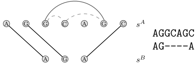
Figure 8: Gaps have to be realized by exactly one gap edge (in this example represented by the solid gray line), and cannot be split into two separate smaller gaps (the two dotted gap edges in this example).
