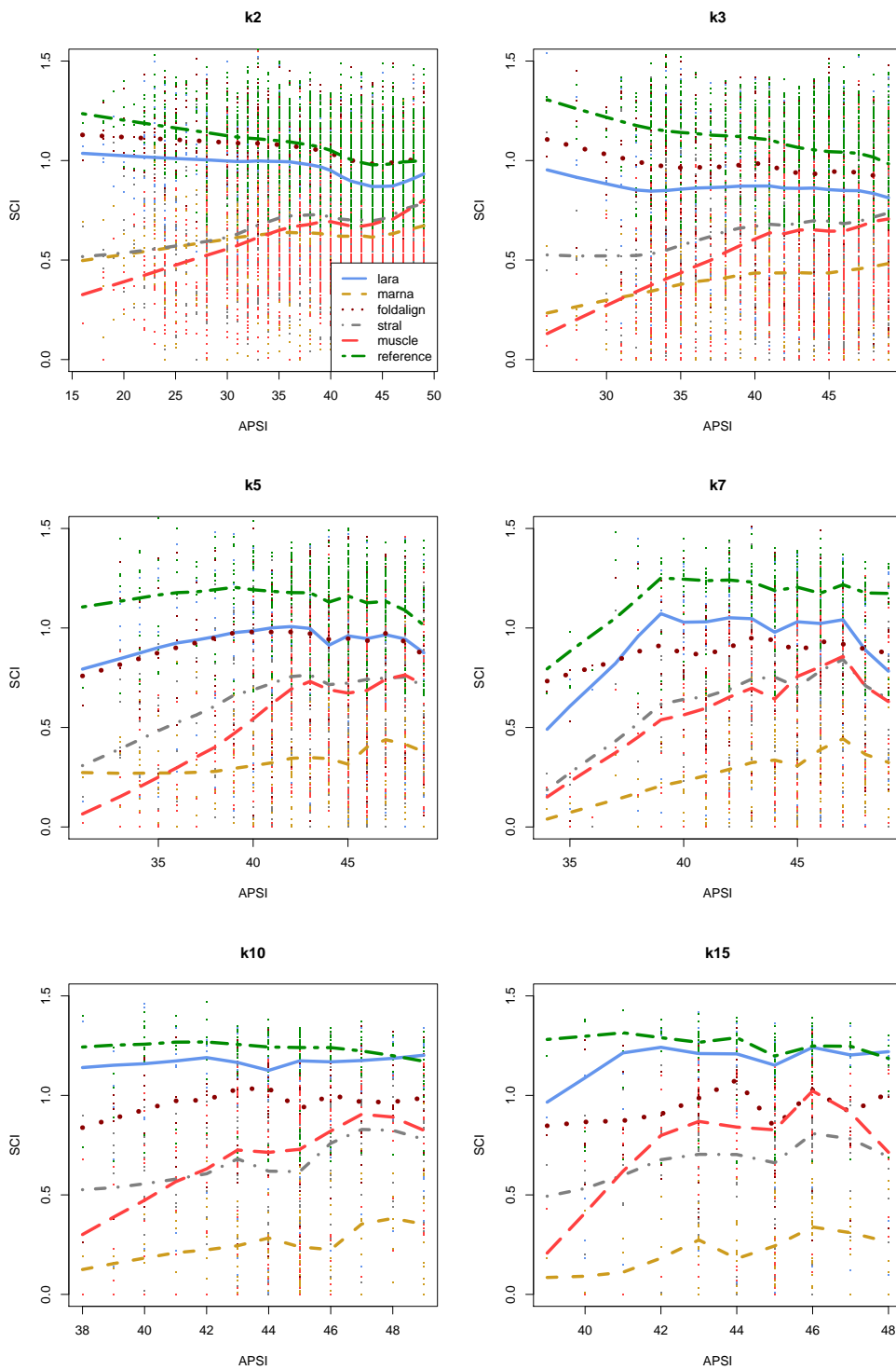
Figure 17: Results on all low homology instances containing 2 (upper left), 3 (upper right), 5 (middle left), 7 (middle right), 10 (lower left), and 15 (lower right) instances from the BRALIBASE benchmark set. The y -axis gives the SCI score. The legend from the upper left plot applies to the other plots as well.
