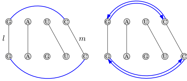
Figure 11: One interaction match is split into two directed interaction matches.
