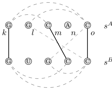
Figure 9: The pairs (k, m) and (k, o) are valid interaction matches. The pair (l, n) , however, is not a valid interaction match since l and n cross each other.
