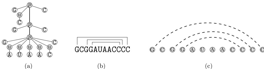
Figure 3: Different models representing RNA structures: (a) tree representation, (b) annotated sequences, and (c) graph-based models.
