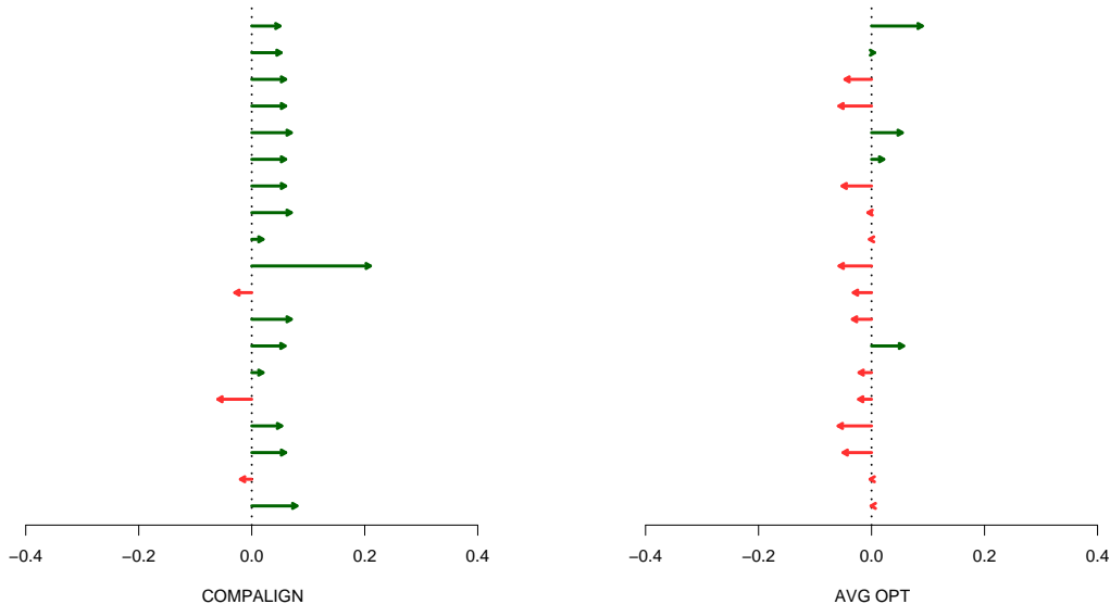
Figure 14: Change of the Compalign score and optimality ratio after changing the scoring from BPP to RIBOSUM matrices for the 19 outlier instances.
