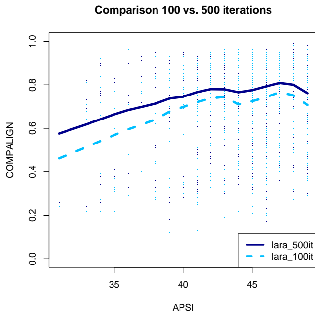
Figure 12: Comparison of all k10 instances of low homology between LARA running 100 or 500 iterations. Each dot corresponds to one problem instance, the thick lines were computed using Lowess regression.
