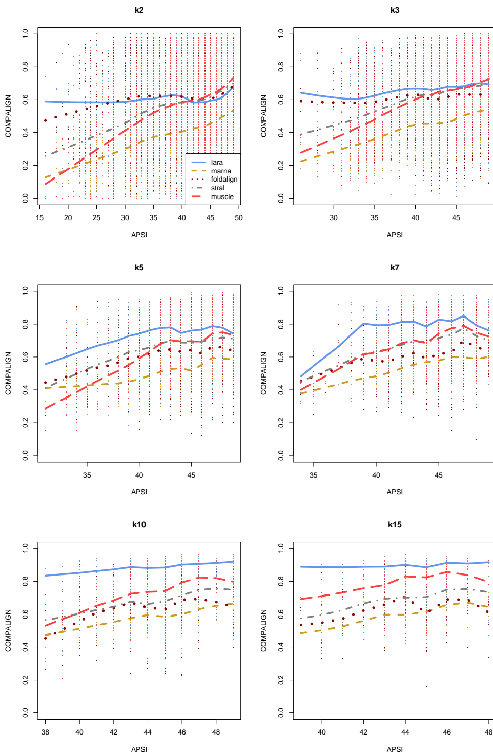
Figure 16: Results on all low homology instances containing 2 (upper left), 3 (upper right), 5 (middle left), 7 (middle right), 10 (lower left), and 15 (lower right) instances from the BRALIBASE benchmark set. The x - and y -axes give the average pairwise sequence identity (APSI) and the Compalign score. The legend from the upper left plot applies to the other plots as well.
