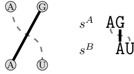
Figure 5: Sequences s^A = AG and s^B = AU are given. The solid line between G and A represent the alignment of these two nucleotides. If we added the gray dashed line, this would induce an ordering conflict.
