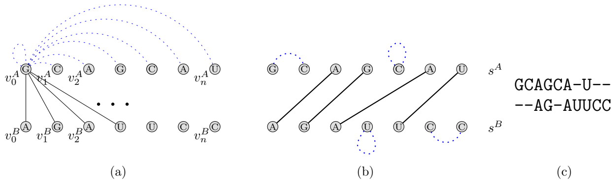
Figure 7: (a) Initial model additionally augmented with gap edges. The figure shows possible alignments edges and all gap edges starting from v_0^A (for sake of clarity, all other gap edges and interaction edges are not displayed). Note, however, that every node has outgoing gap edges to all other nodes in the sequence. The subset of lines and gap edges (b) corresponds to the alignment (c).
