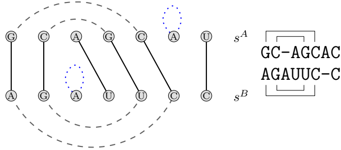
Figure 10: Valid gapped structural trace: every vertex is incident to exactly one line or is spanned by a gap edge. There are no crossing lines, and every line is incident to at most one interaction match.
