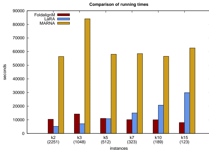
Figure 18: The plot shows a comparison of the running times between the structural programs tested. With an increasing number of input sequences, a progressive alignment strategy pays off compared to the computation of all pairwise alignments. The numbers in brackets denote the number of instances per input class.
