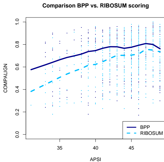
Figure 15: Comparison between base pair probability (BPP) and RIBOSUM scoring.
