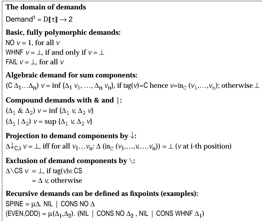
Figure 3. Demands and Demand Operators
